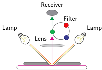
Fig. 2. Colorimeter operation.
