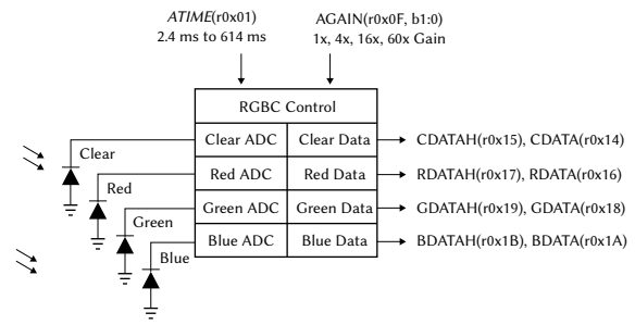
Fig. 6. RGBC operation.
