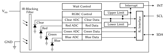
Fig. 5. Sensor functional block diagram (TCS34725 Datasheet).
