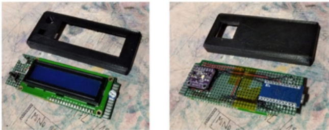
Fig. 9. Colorimeter assembly.
