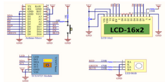
Fig. 8. Schematic of the electronic assembly.
