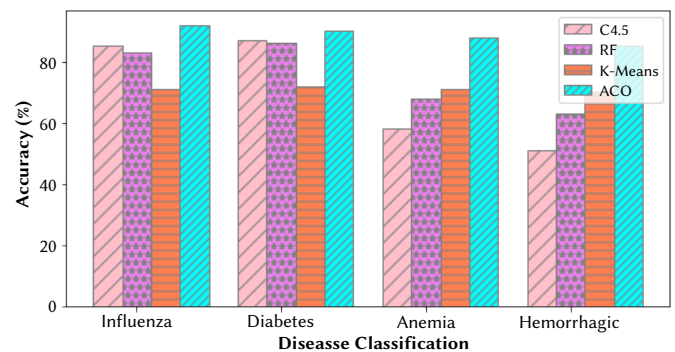
Fig. 5. Disease Classification Comparison.
