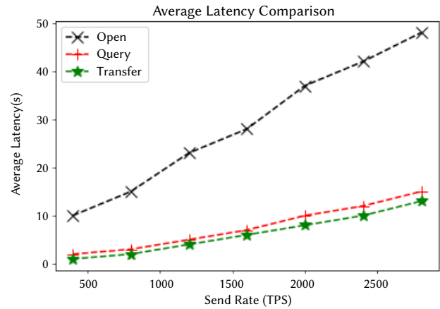
Fig. 8. Latency Time Analysis.
