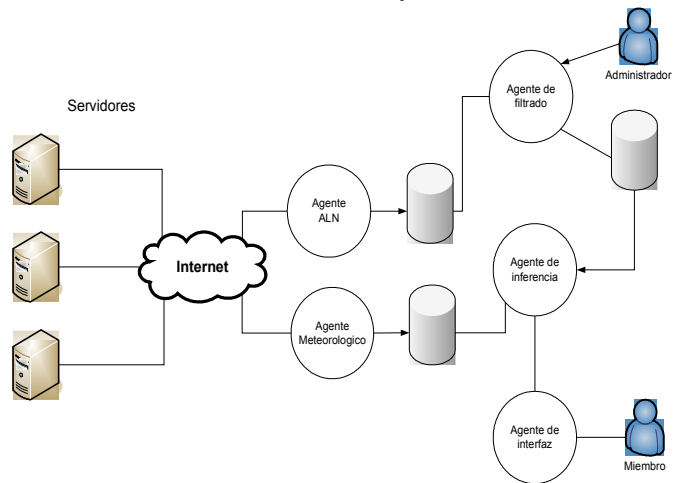
Fig. 3. Agents diagram
