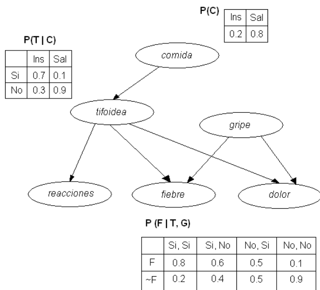
Fig. 1. Example fo bayesian network with some parameters
